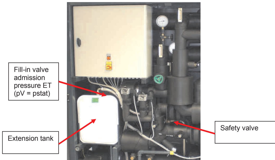
Photo: Safety subassembly
