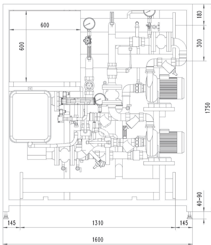
Figure CoolTrans 100 (Standard) front view
