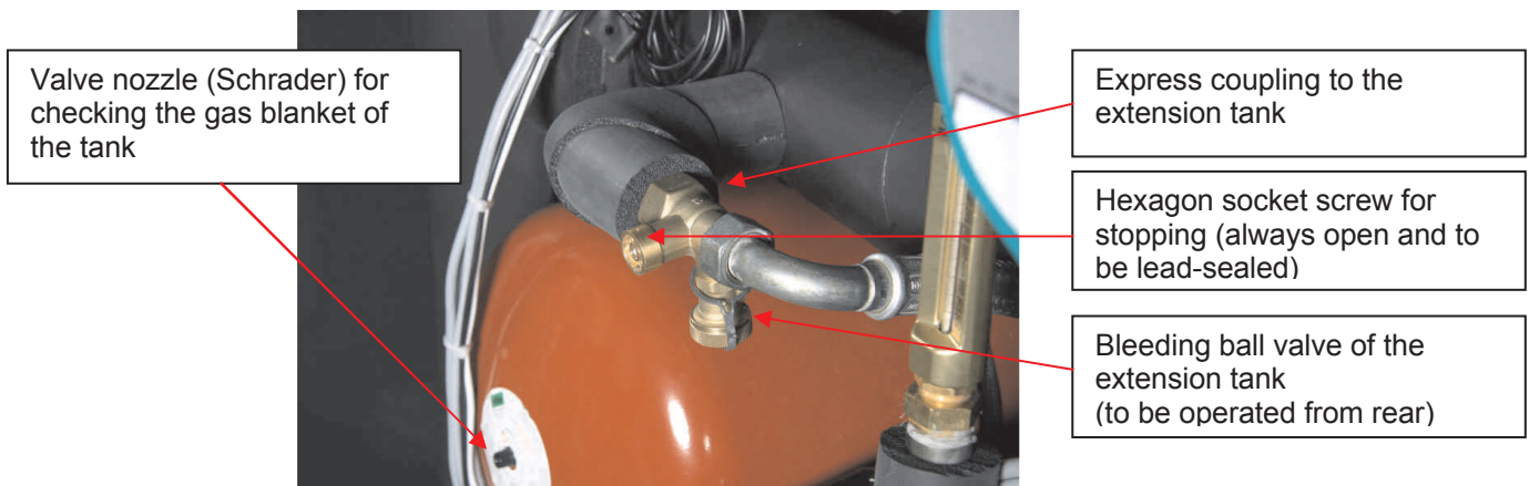
Photo: Membrane extension tank with express coupling
