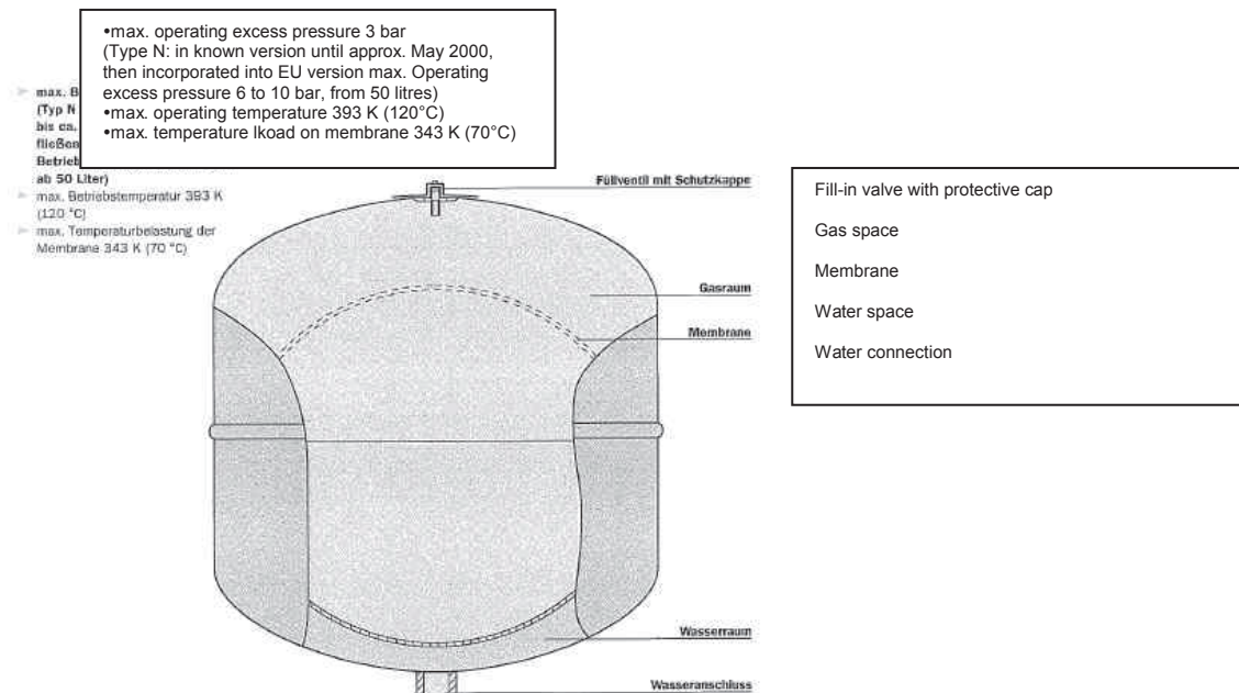
Figure: Cross-section of the membrane extension tank
