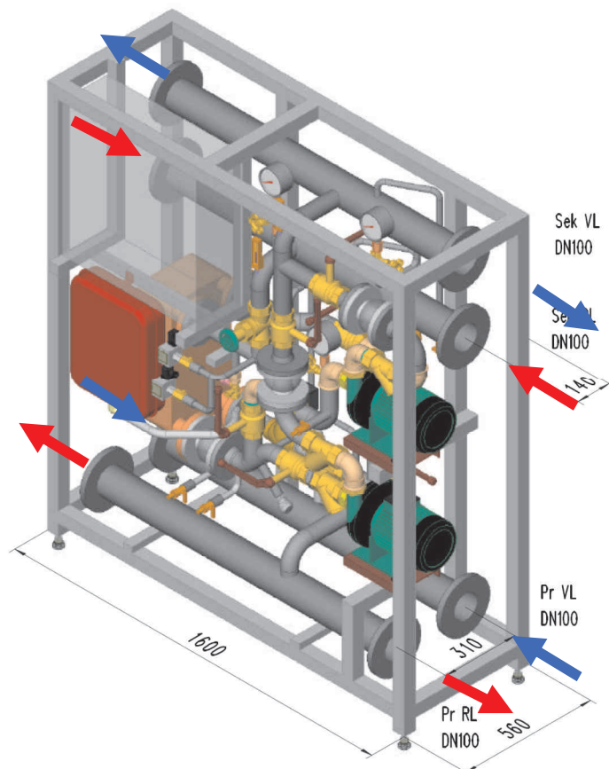
Figure CoolTrans 100( threeD)
